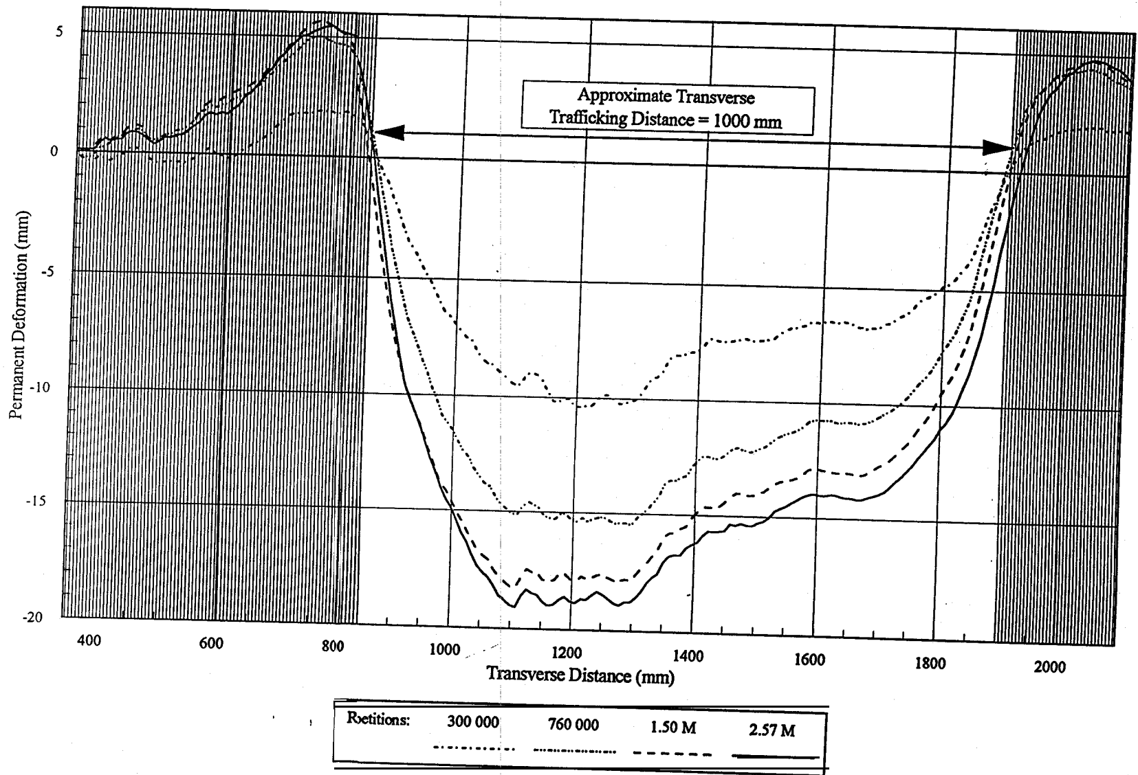
Figure 9. Point 15 rofilometer Cross-section and Final Straight Edge Measurement
