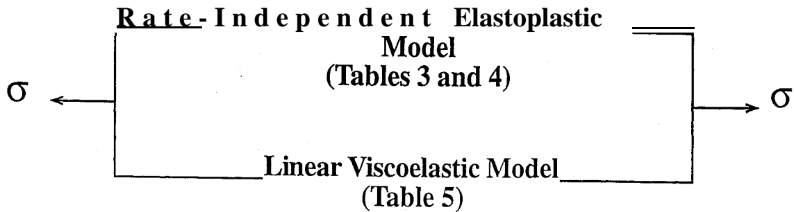
Figure 3. Constitutive Relationship Concept, One Dimensional Schematic
