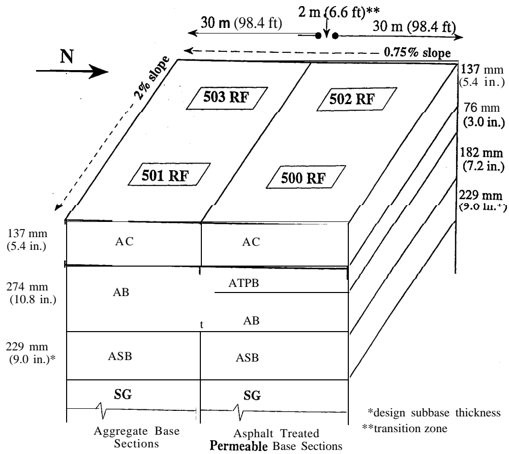
Figure 8. Test Pavements
