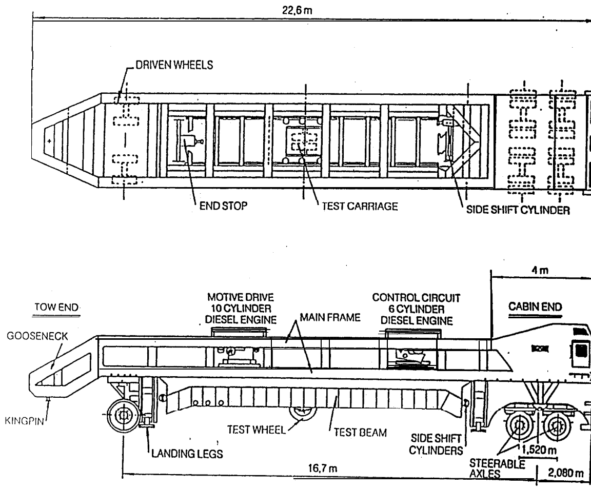
Figure 2. Line Diagram of the Heavy Vehicle Simulator (HVS)
